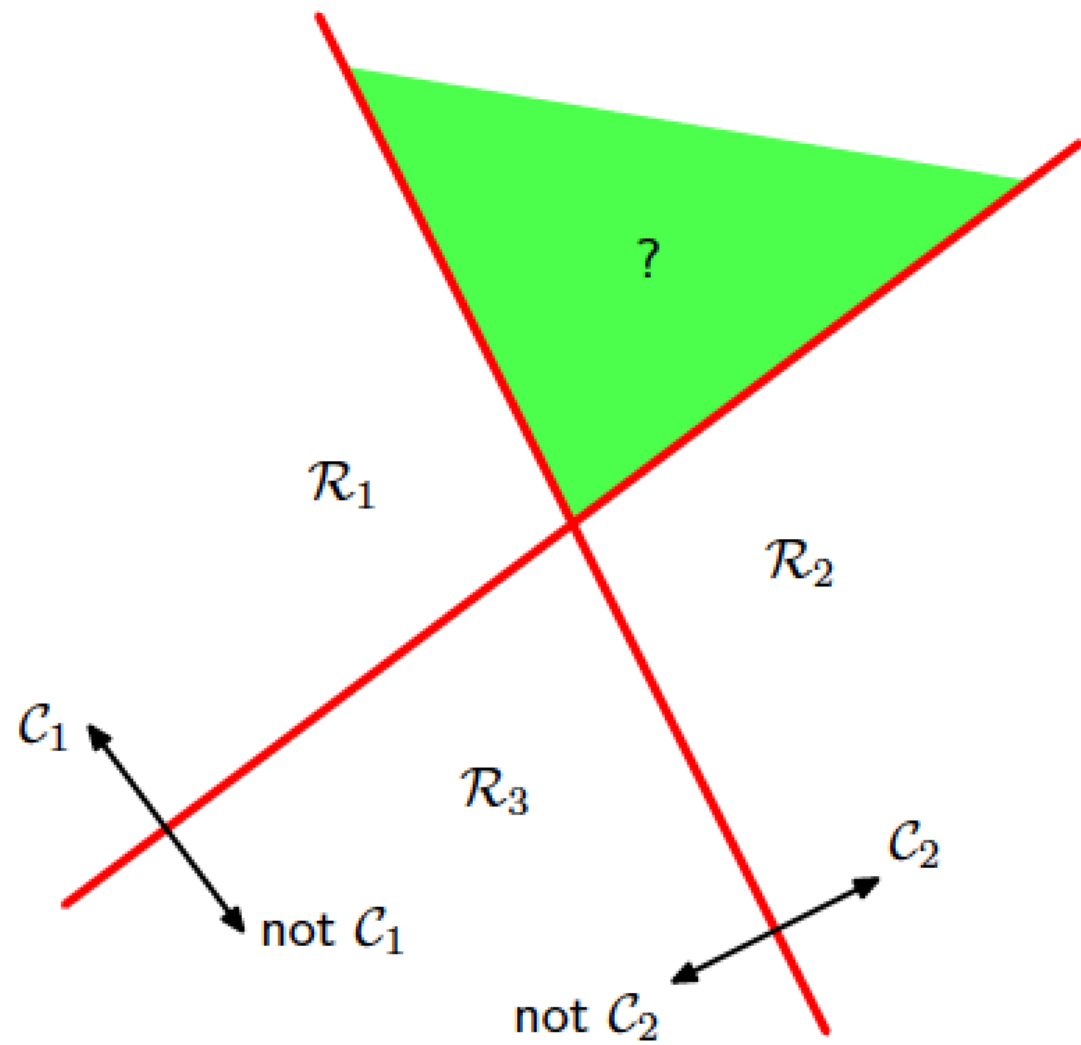
Figure 4.2 Attempting to construct a K class discriminant from a set of two class discriminants leads to ambiguous regions, shown in green. On the left is an example involving the use of two discriminants designed to distinguish points in class C_k from points not in class C_k . On the right is an example involving three discriminant functions each of which is used to separate a pair of classes C_k and C_j .
