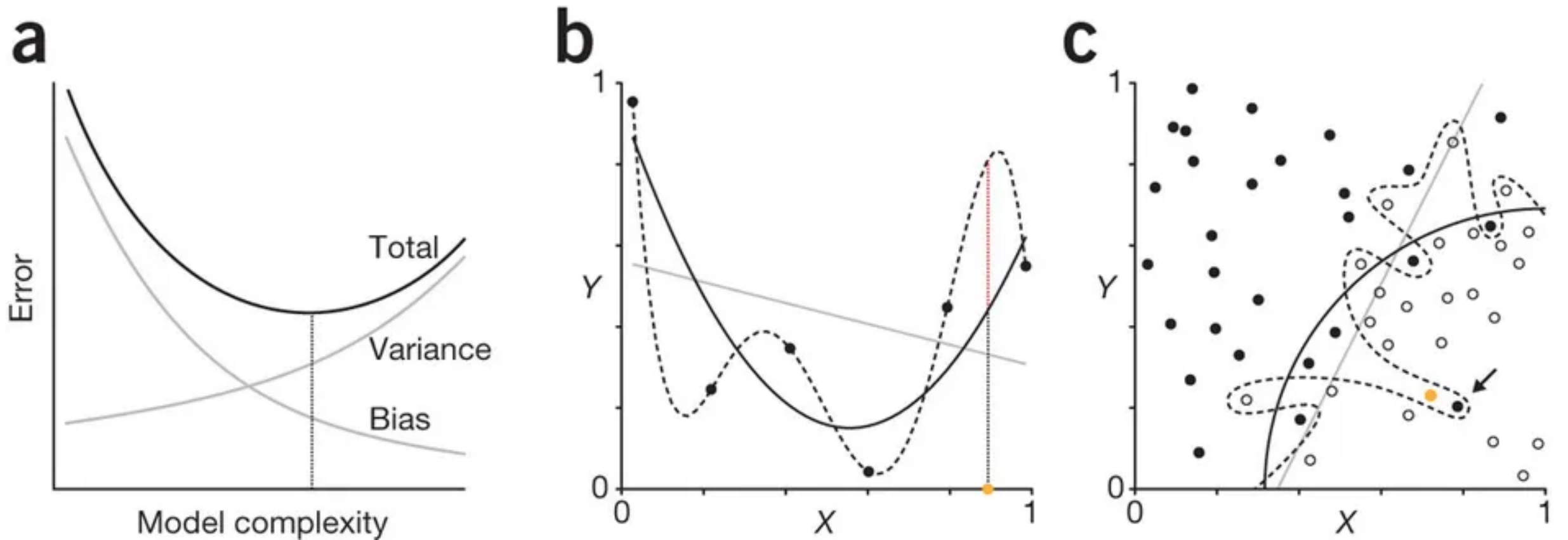
(a) When model complexity increases, generally bias decreases and variance increases. The choice of model complexity is informed by the goal of minimizing the total error (dotted vertical line). (b) Polynomial fits to data simulated from a third-order polynomial underlying a model with normally distributed noise. The fits shown exemplify underfitting (gray diagonal line, linear fit), reasonable fitting (black curve, third-order polynomial) and overfitting (dashed curve, fifth-order polynomial). There is a large difference (red dotted line) in Y prediction at X = 0.9 (orange circle) between the reasonable and overfitted models. (c) Two-class classification (open and solid circles) with underfitted (gray diagonal line), reasonable (black curve) and overfitted (dashed curve) decision boundaries. The overfit is influenced by an outlier (arrow) and would classify the new point (orange circle) as solid, which would probably be an error.
